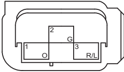
FF7 Front Parking Radar Sensor R
