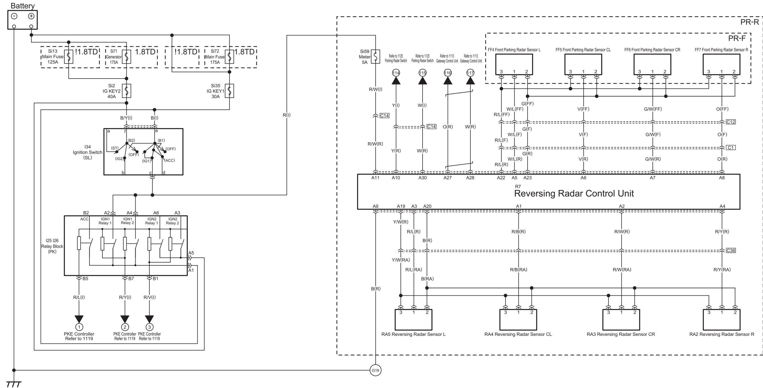
R7 Reversing Radar Control Unit
