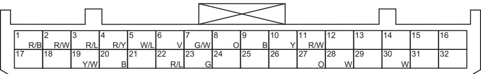
FF5 Front Parking Radar Sensor CL
