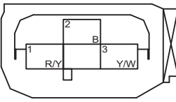
RA2 Reversing Radar Sensor R
