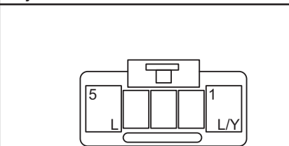
DS7 Seatback Forward/Backward Adjustment Motor (Driver Side)
