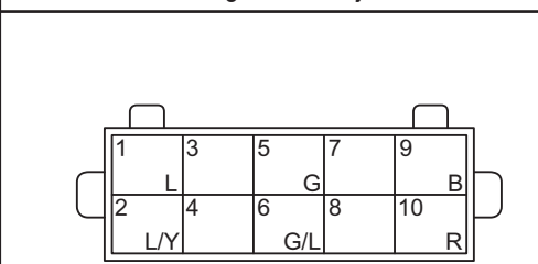
FPS4 Front Passenger Seat Adjustment Switch
