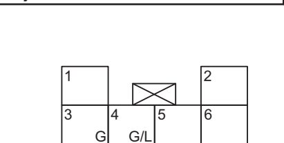
DS5 Seat Forward/Backward Adjustment Motor (Driver Side)
