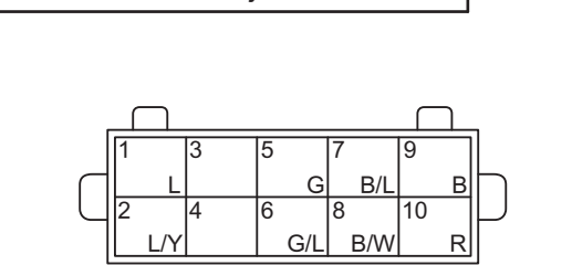
DS4 Driver Seat Adjustment Switch
