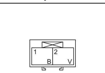
DS6 Seat Heating Cushion (Driver Side)
