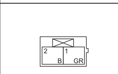
DS1 Seat Belt Buckle Switch (Driver Side)
