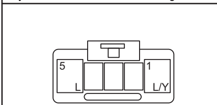
FPS6 Seatback Forward/Backward Adjustment Motor (Front Passenger Side)
