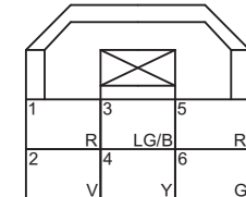
RR1 Window Motor (Rear Door RH)
